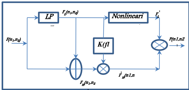
Fig. 2 System used for IR image enhancement using nonlinearity.
