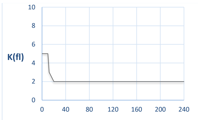
Fig. 2 Function k(f_L) used in the processing [13].
